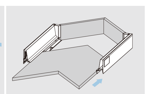
Bottom assembly
