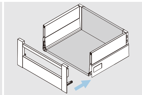
Front assembly
