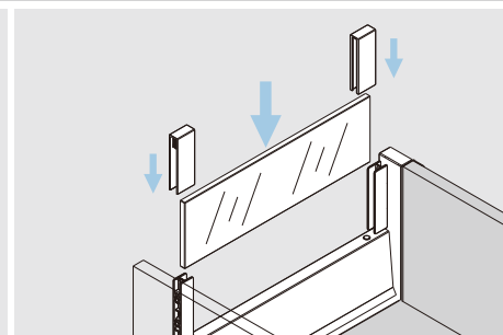
Side assembly
