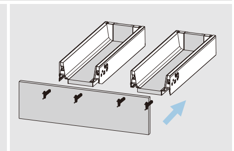
Front assembly
