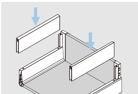
Side assembly
