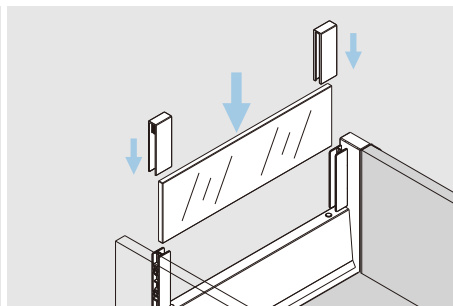
Side assembly
