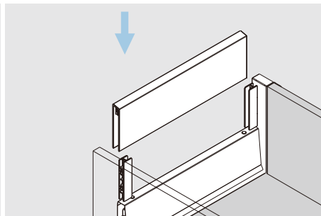
Side assembly
