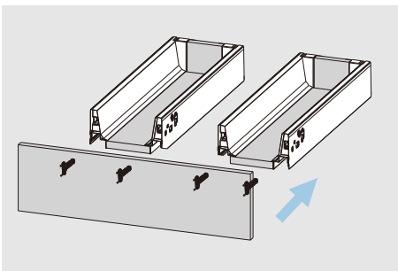
Front assembly
