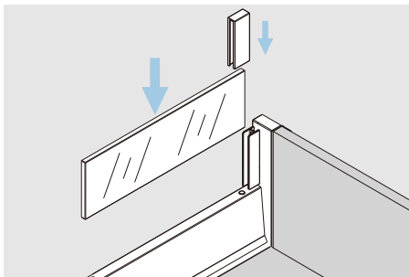
Side assembly
