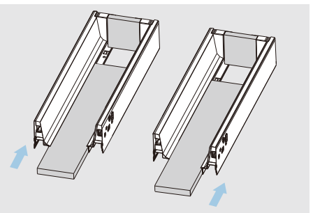
Bottom assembly
