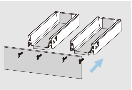
Front assembly
