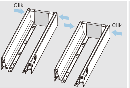
Back assembly
