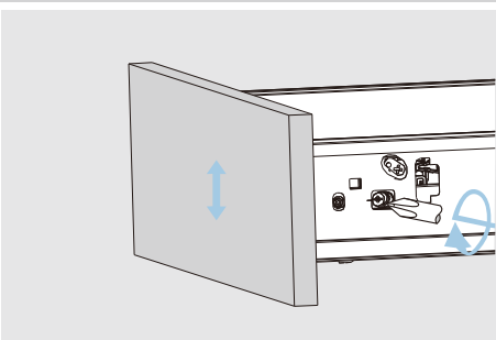
Up&down adjustment
