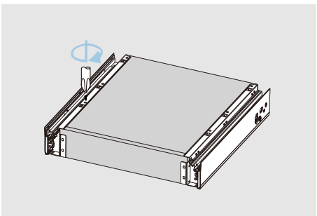
Fix screws
