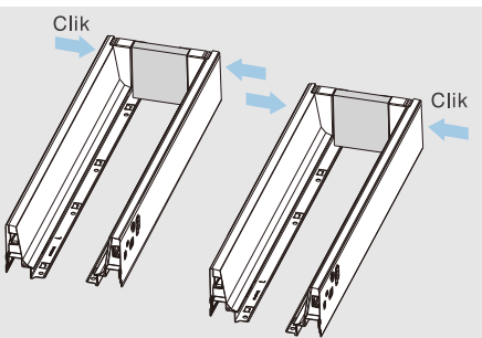
Back assembly
