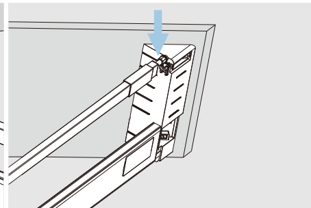
Front assembly
