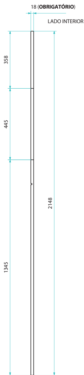
PORMENOR - U (1:6)
