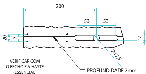
PORMENOR - U (1:6)
